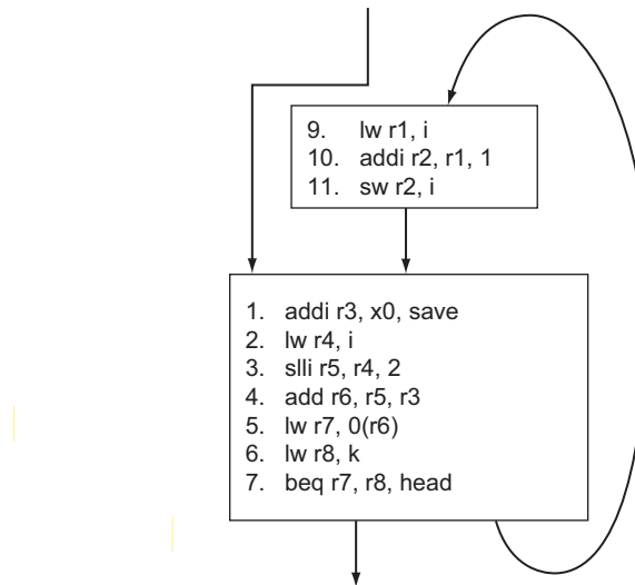
FIGURE e2.15.4 A control flow graph for the while loop example. Each node represents a basic block, which terminates with a branch or by sequential fall-through into another basic block that is also the target of a branch. The IR statements have been numbered for ease in referring to them. The important transformation performed was to move the while test and conditional branch to the end. This eliminates the unconditional branch that was formerly inside the loop and places it before the loop. This transformation is so important that many compilers do it during the generation of the IR. The mul was also replaced with (“strength-reduced to”) an slli .
