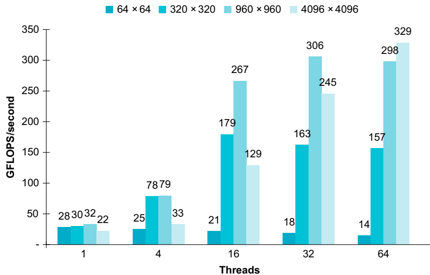
FIGURE 6.33 DGEMM performance versus the number of threads for four matrix sizes. The performance improvement compared to the original C code in Figure 3.20 for the 960 x 960 matrix with 32 threads is an astounding 152 times faster!
